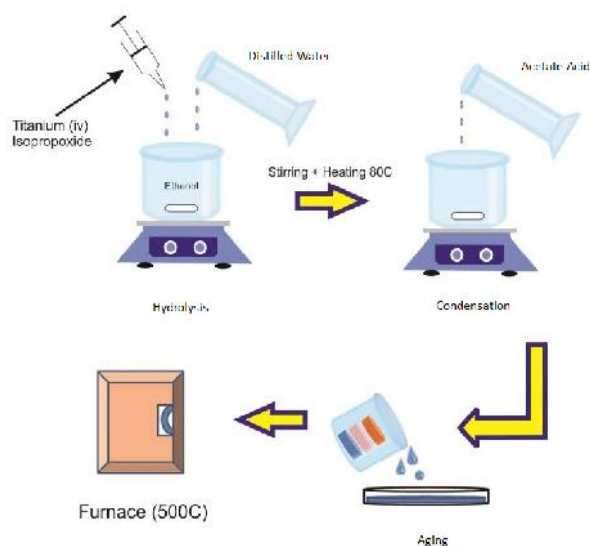
Fig. 1. Sol-Gel Process (Hydrolysis, Condensation, and Aging).
